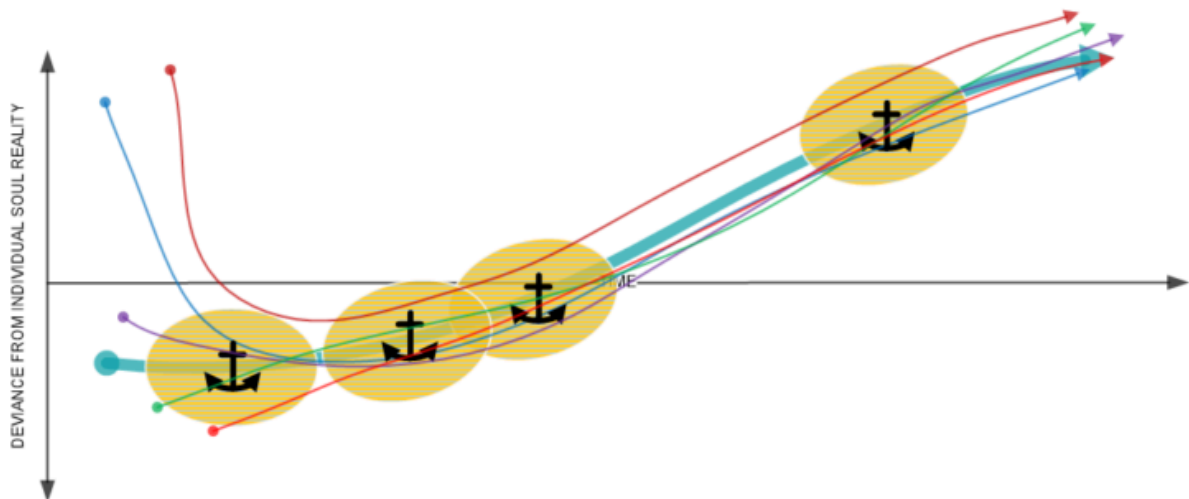
How the anchored path looks with avoidance.
