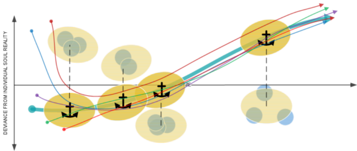
World-lines following an anchored path.
